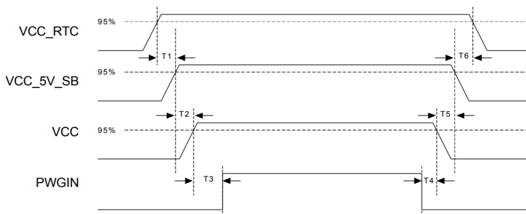
Figure 12: Power Input Sequencing
