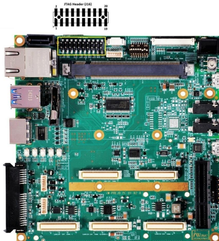
Figure 20: JTAG Header
