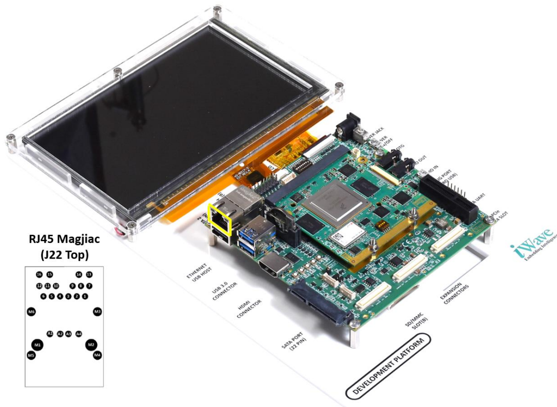
Figure 9: RJ45 Magjack
