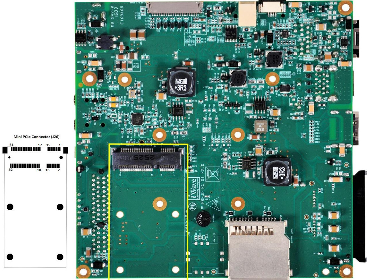
Figure 6: Mini PCIe Connector
