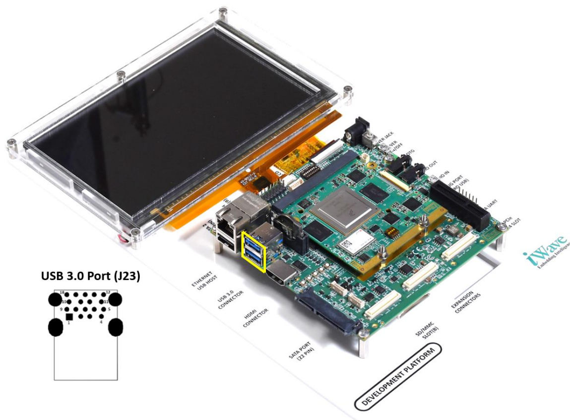
Figure 8: USB3.0 Host
