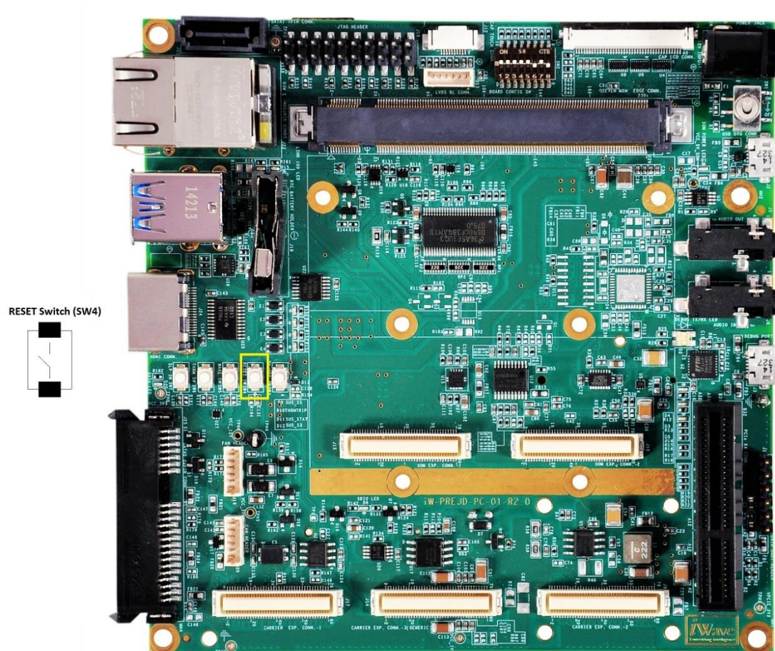
Figure 22: Reset Switch
