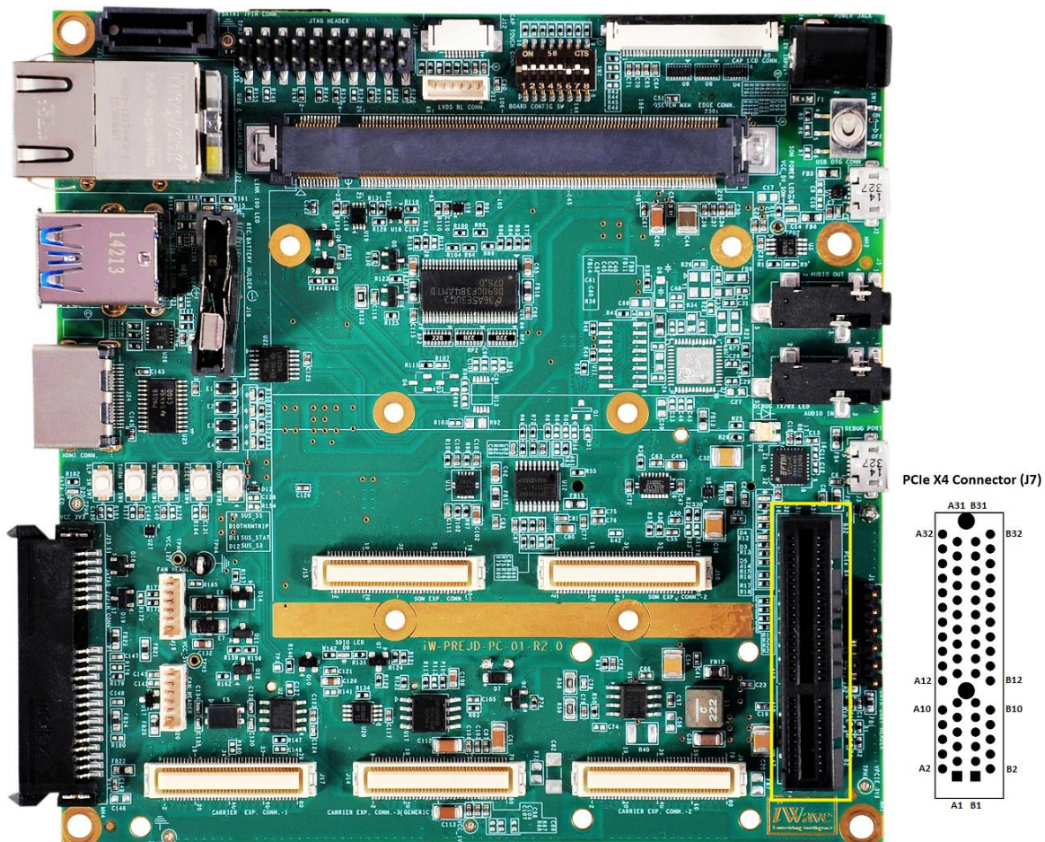
Figure 5: PCIe4 Connector
