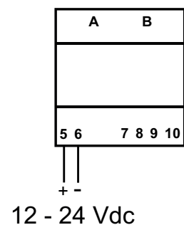
Fig. 14 Power supply
