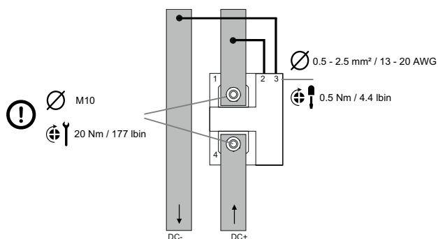
Fig. 10 Current (option A) and voltage inputs
