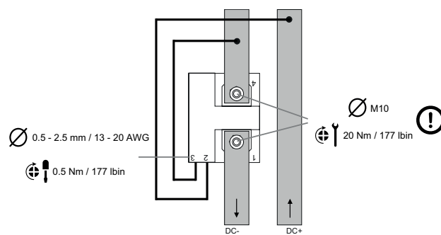
Fig. 11 Current (option B) and voltage inputs
