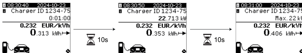
Fig. 9 Charging session in progress, with TT field, system power, custom string 1 and 2 active. Time trigger is set to 10 seconds.
