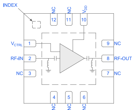
Figure 1. TSS-14252LN+ Functional Diagram
