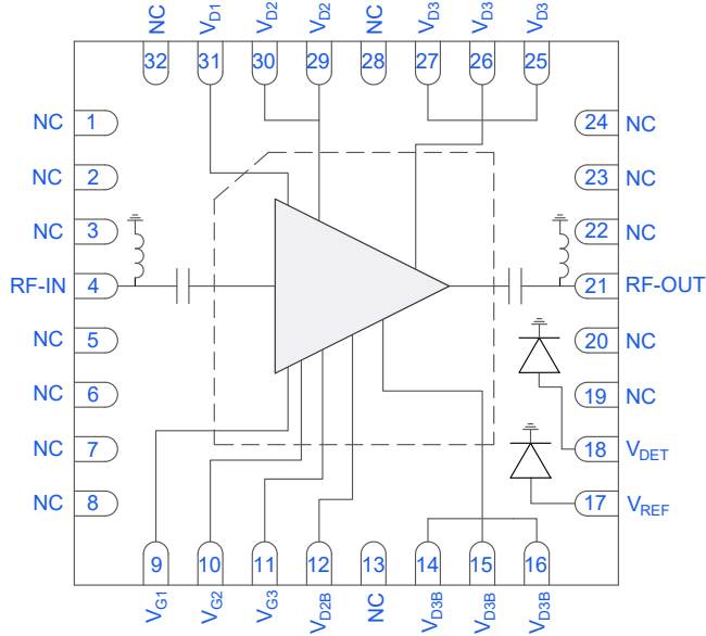
Figure 1. PMA5-123-3W+ Functional Diagram
