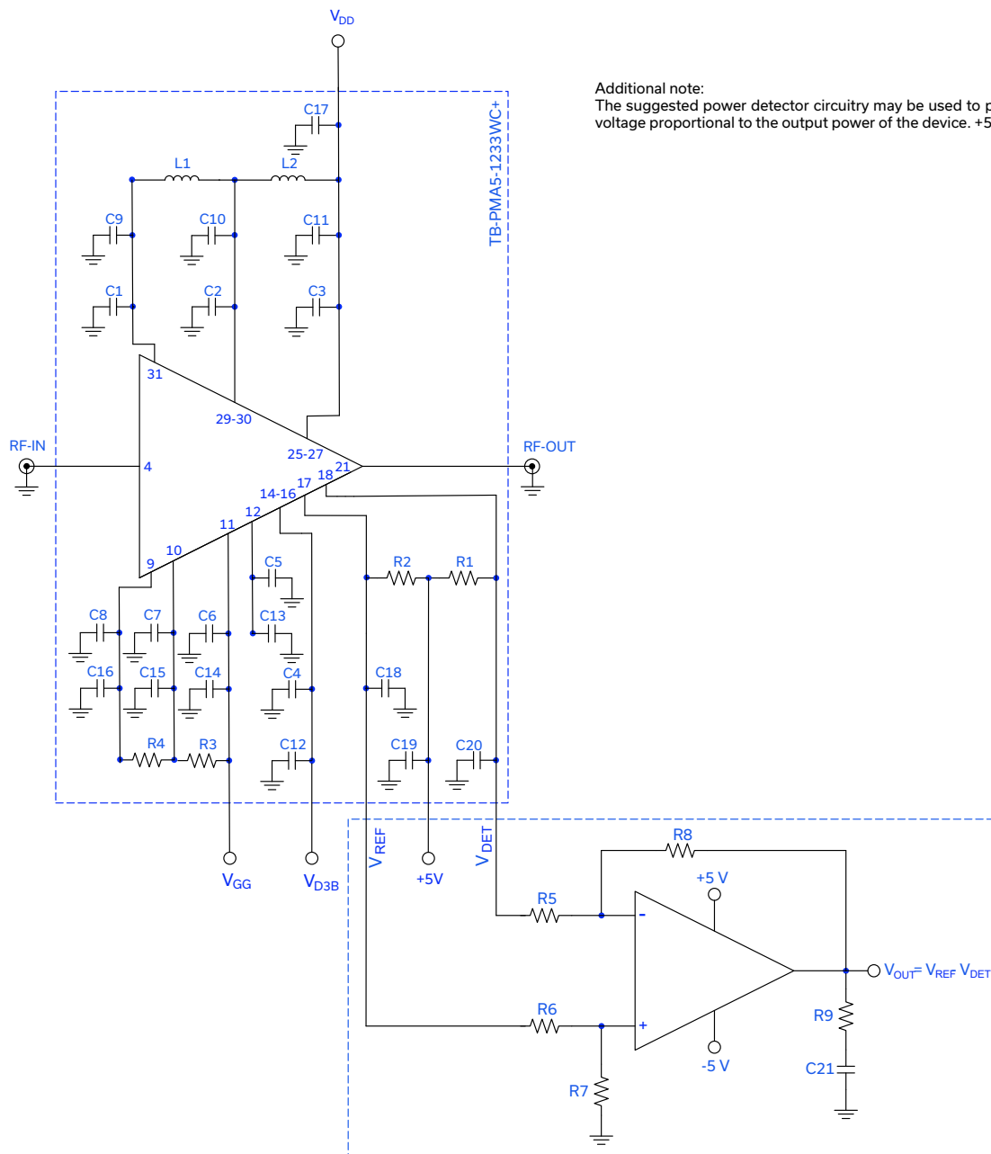
Figure 3. PMA5-123-3W+ Characterization Circuit with Power Detector Circuitry
