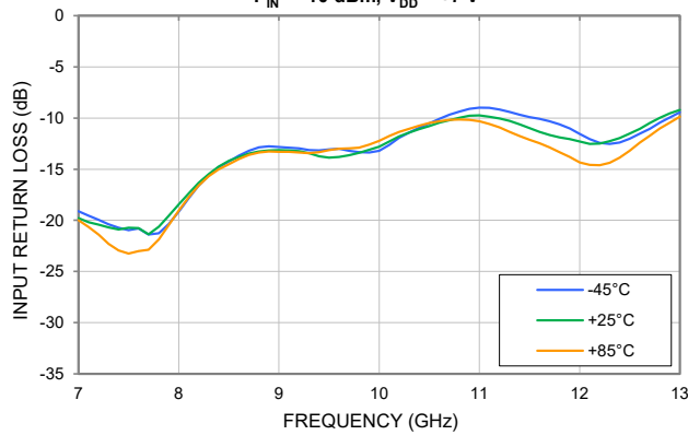
INPUT RETURN LOSS vs. TEMPERATURE
