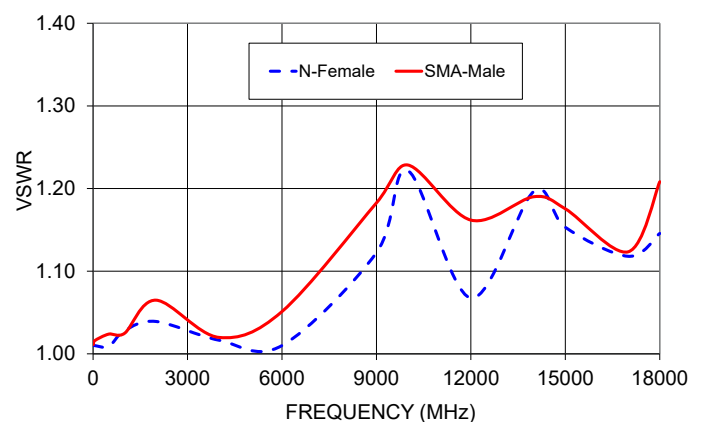
NFFL-SM50+ VSWR
