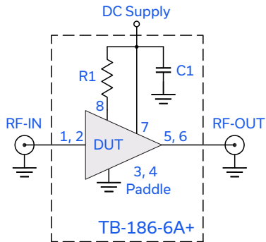
Fig 1. Block Diagram of Test Circuit used for characterization. (DUT soldered on Mini-Circuits Characterization test board TB-186-6A+) Gain, Return Loss, Output Power at 1 dB Compression (P1 dB), Output IP3 (OIP3) and Noise Figure measured using Agilent's N5242A PNA-X microwave network analyzer.
