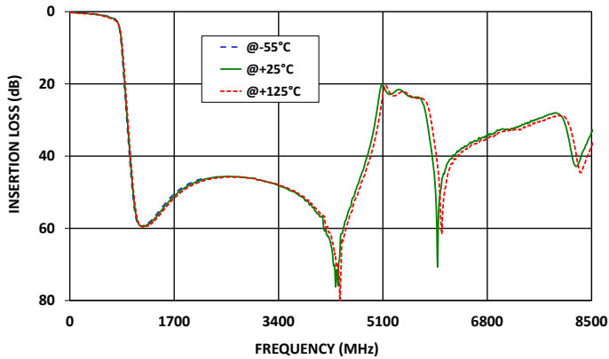
LFCG-630+ INSERTION LOSS
