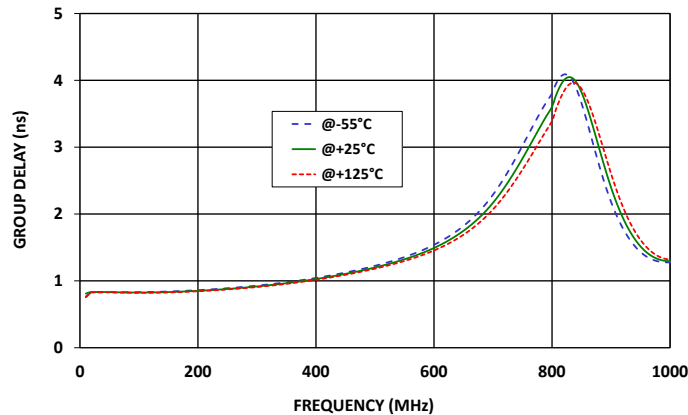
LFCG-630+ GROUP DELAY
