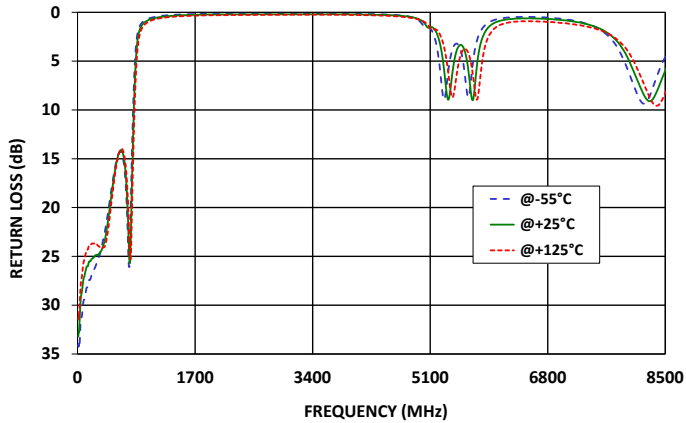
LFCG-630+ RETURN LOSS
