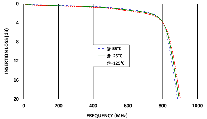
LFCG-630+ INSERTION LOSS (Zoomed)
