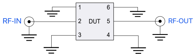
Fig 1. Block diagram of Test Circuit used for characterization, Test board TB-934-2C+ Conditions: Attenuation, VSWR: P_{IN} = 0 dBm
