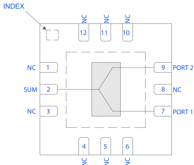
Figure 1. GP2SA+ Functional Diagram
