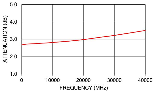
BW-KM3-2W44+ ATTENUATION
