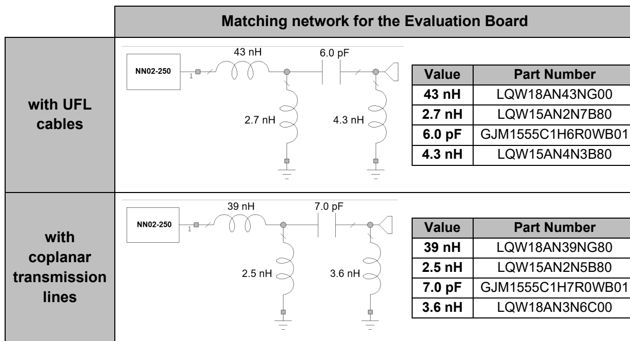
Figure 2 – Matching networks for the LTE700, 1 port configuration.
