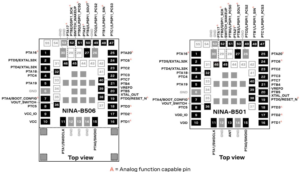
Figure 4: NINA-B50 pin assignments – top view showing NINA-B506 (left) and NINA-B501 (right)
