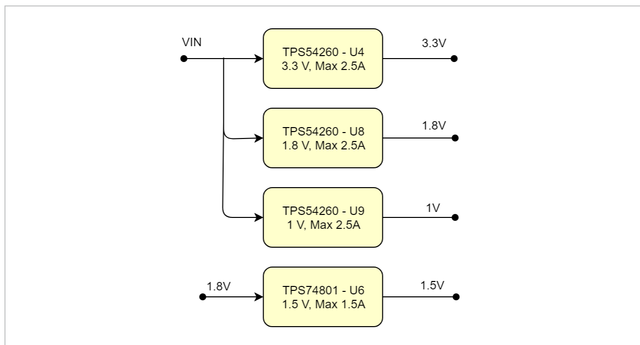
Figure 3: Power Dependencies
