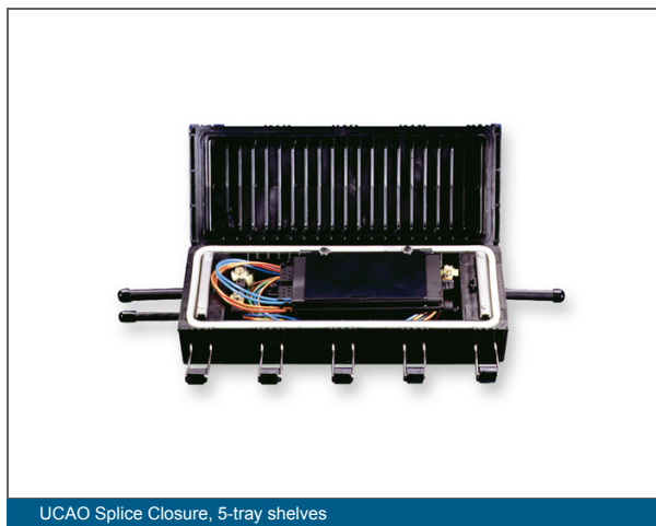
UCAO Splice Closure, 5-tray shelves
