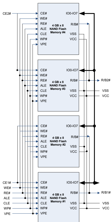
Figure 3. Block Diagram — 16 Gb (4 Gb x 4) with 2 CE#
