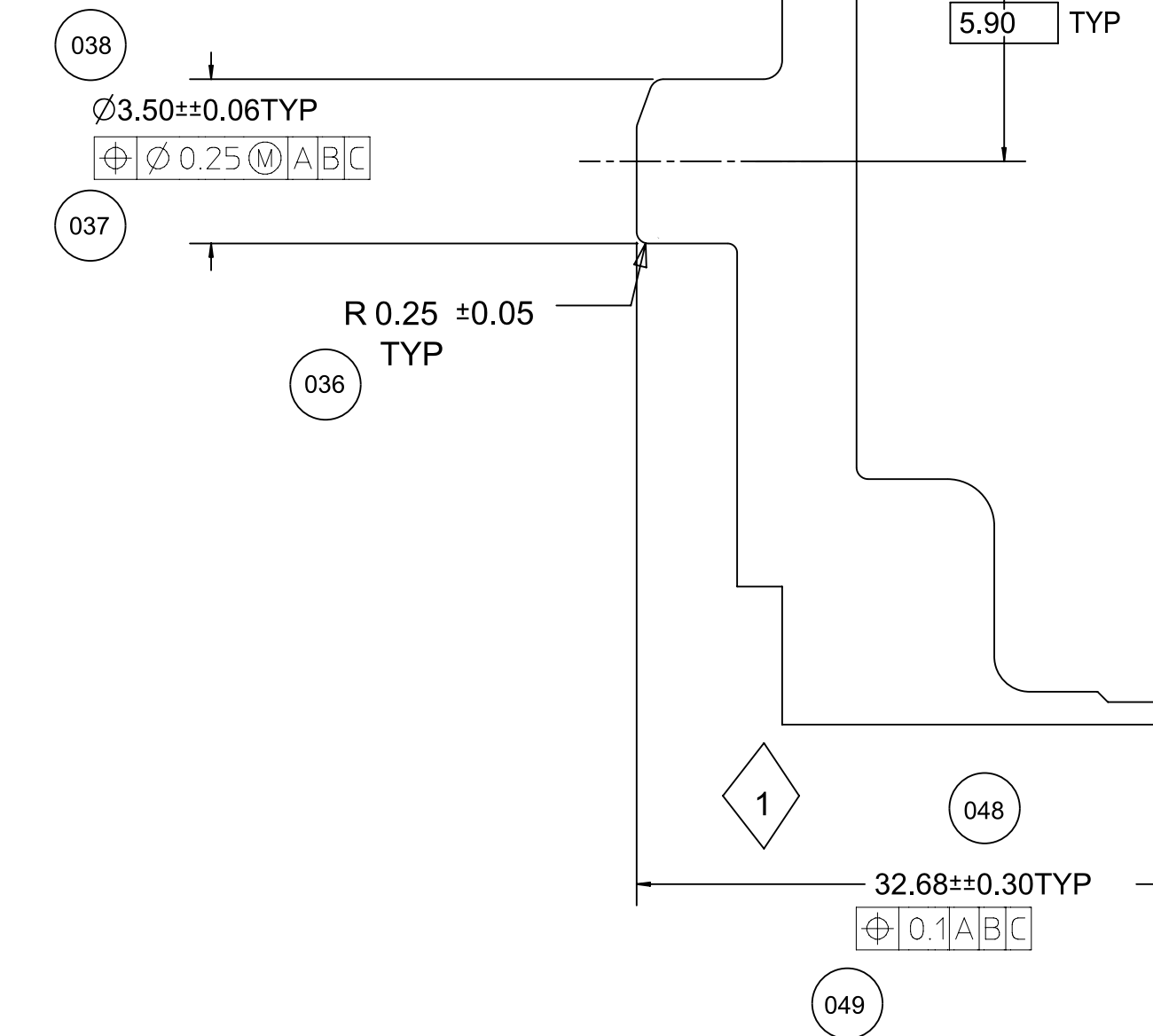
SECTION G-G (CAM POST)
