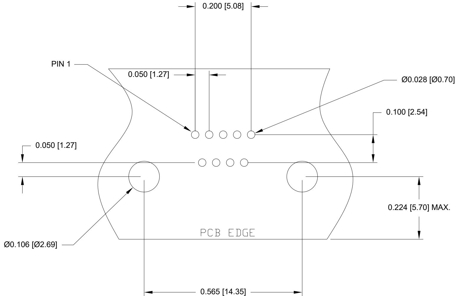
RECOMMENDED RECOMMENDED PCB LAYOUT (Top View) (9 POSITION ONLY) TOLERANCE \pm 0.002 [ \pm 0.05 ]
