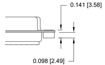
04 ..... 0.065" (SOLDER SIDE)
