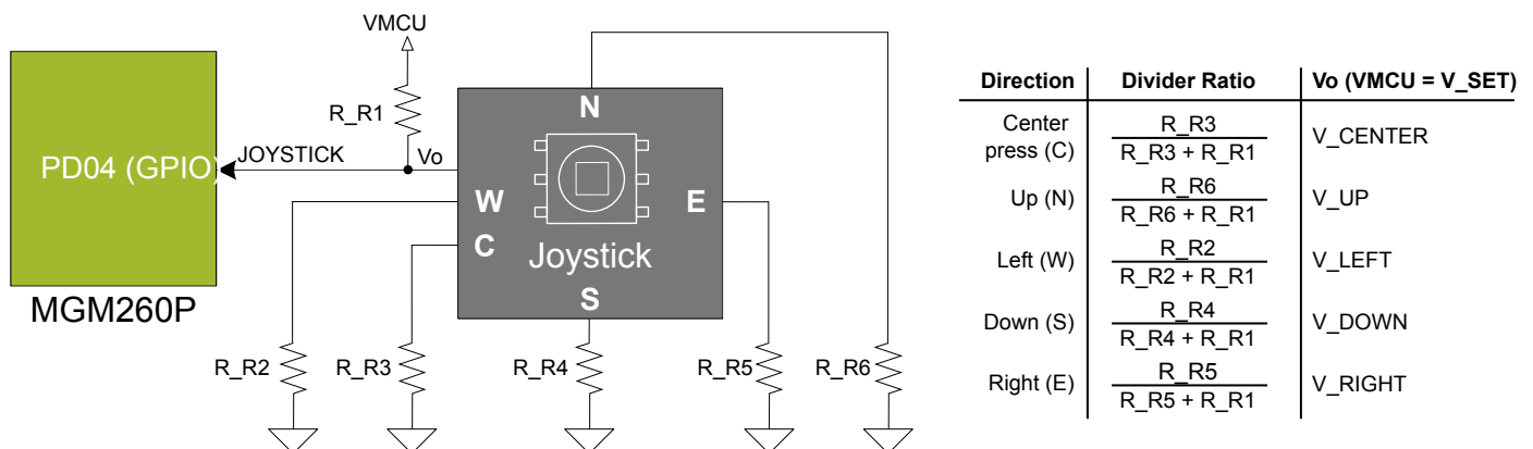
Figure 5.2. Joystick
