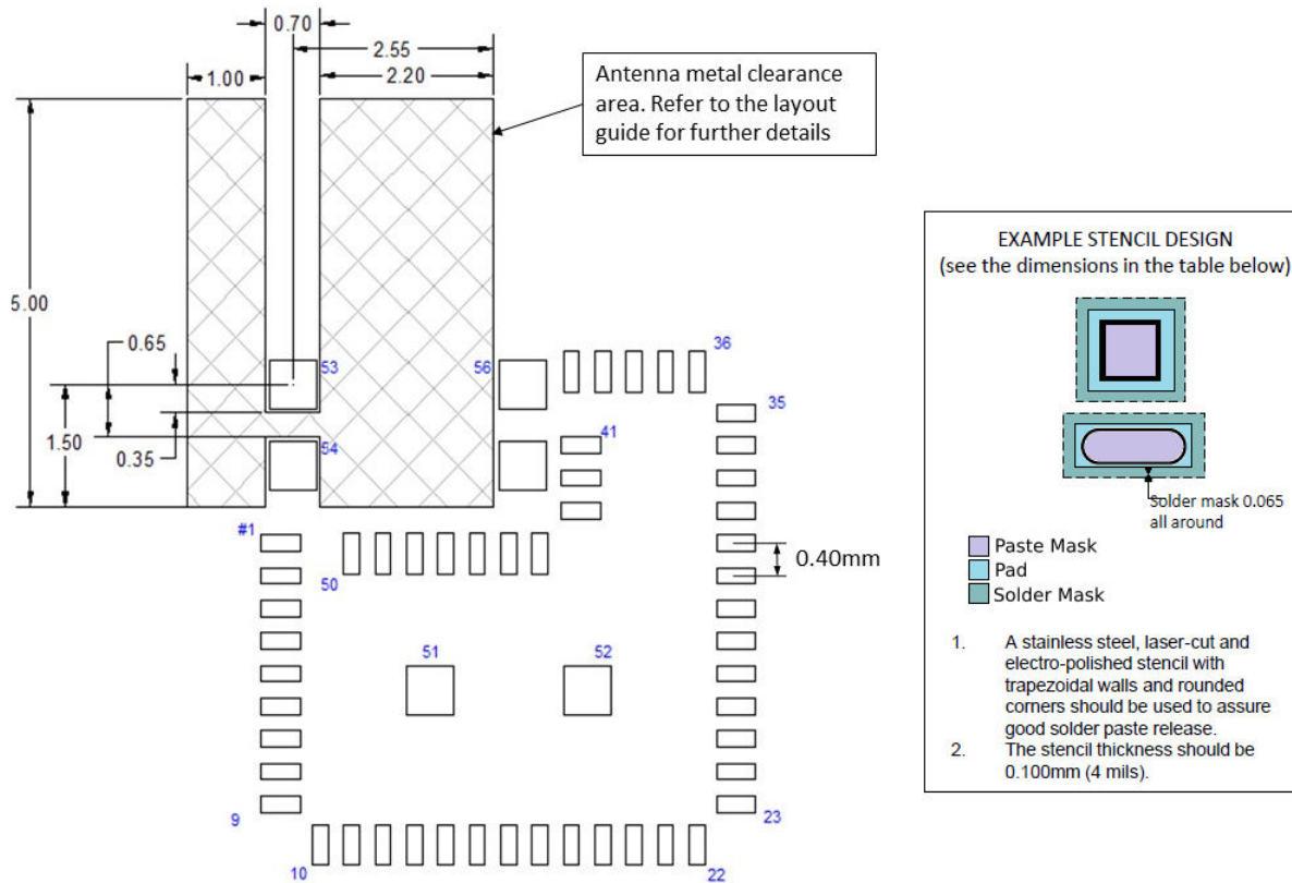
Figure 8.4. BGM11S Recommended Land Pattern
