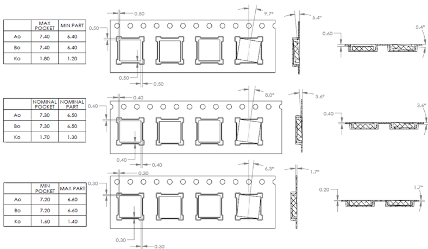
Figure 9.3. Tape information
