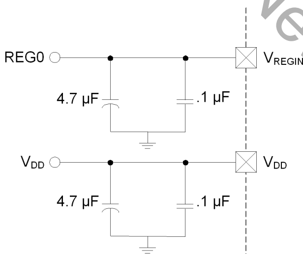
Figure 9.1. External Capacitors for Voltage Regulator Input/Output—Regulator Enabled
