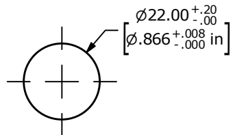
RECOMMENDED PANEL CUTOUT MAX. PANEL THICKNESS 10.0 [.39 in]
