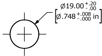
RECOMMENDED PANEL CUTOUT MAX. PANEL THICKNESS 10mm [.39 in]
