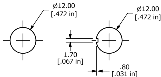
RECOMMENDED PANEL CUT-OUTS
