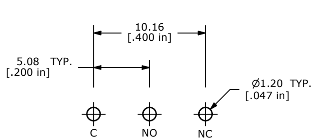
P.C. MOUNTING
