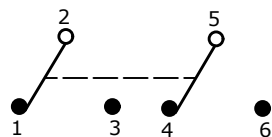
▲CIRCUIT: DPDT
