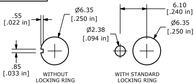
RECOMMENDED PANEL MOUNTING
