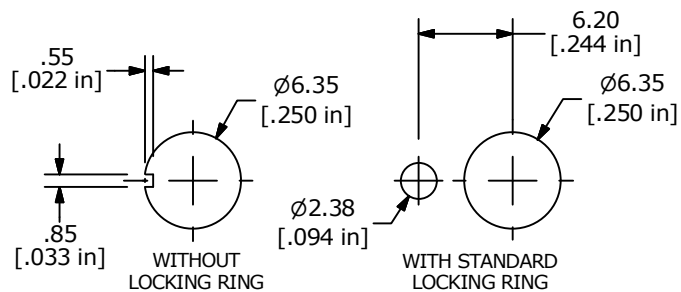
RECOMMENDED PANEL MOUNTING
