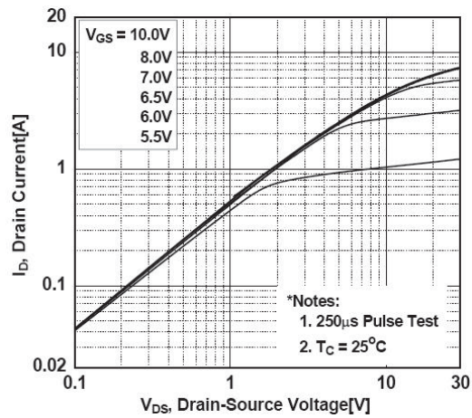
Fig. 1 On-State Characteristics
