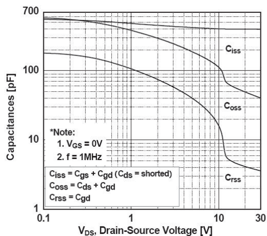
Fig. 5 Capacitance Characteristics
