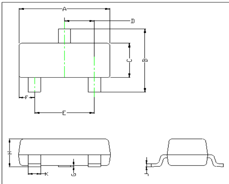
SOT23 Package Outline
