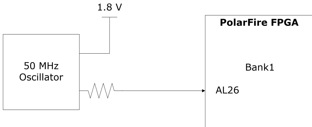
Figure 16 • 50 MHz Oscillator Interface
