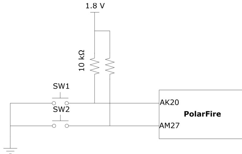
Figure 20 • Push-Button Interface
