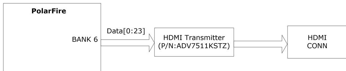
Figure 6 • HDMI1.4 Interface
