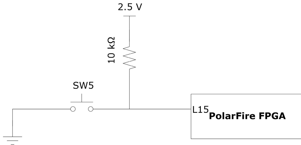
Figure 17 • Device Reset
