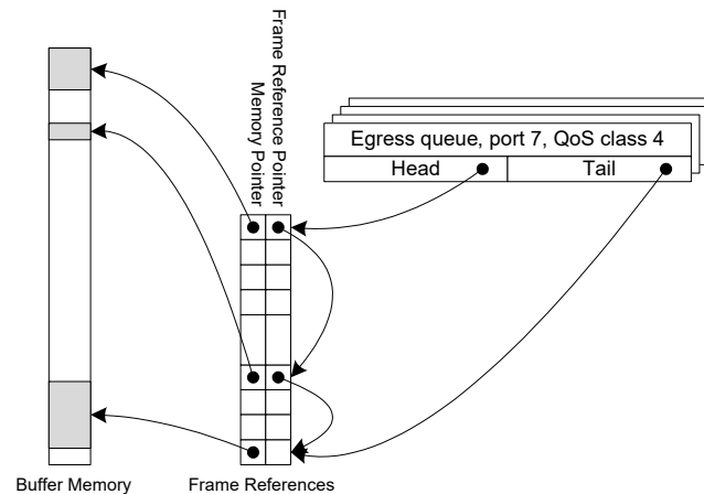
FIGURE 2-31: FRAME REFERENCE
