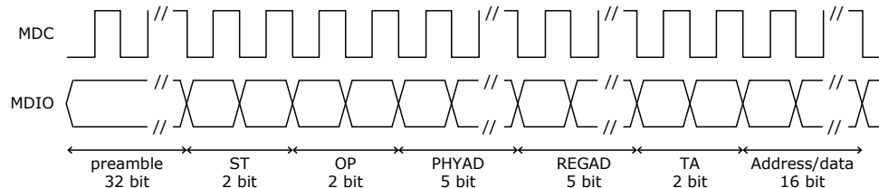
FIGURE 3-25: MII MANAGEMENT TIMING
