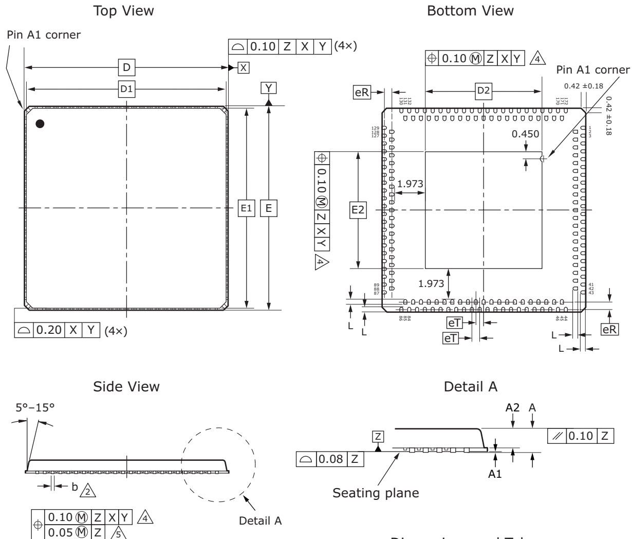
FIGURE 8-1: PACKAGE DRAWING
