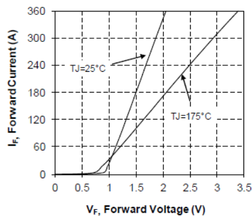
Figure 18 • Forward Characteristics
