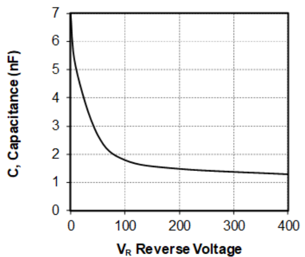
Figure 1-17. Capacitance vs. Reverse Voltage
