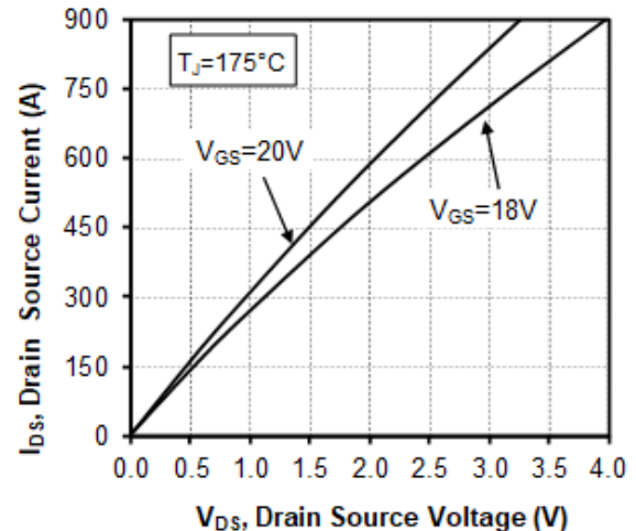
Figure 1-3. Output Characteristics, T J = 175 °C
