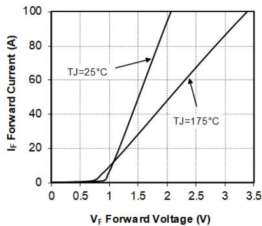
Figure 1-16. Forward Characteristics
