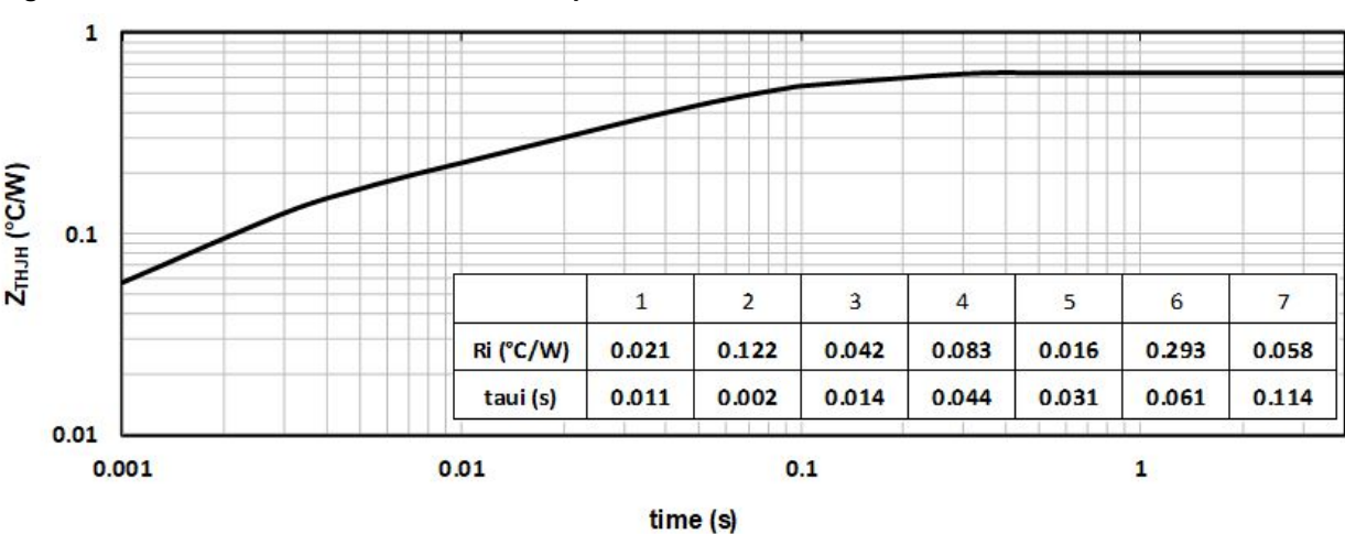
Figure 1-15. Junction-to-Heatsink Thermal Impedance
