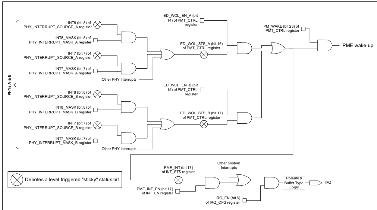
FIGURE 6-1: PME INTERRUPT SIGNAL GENERATION
