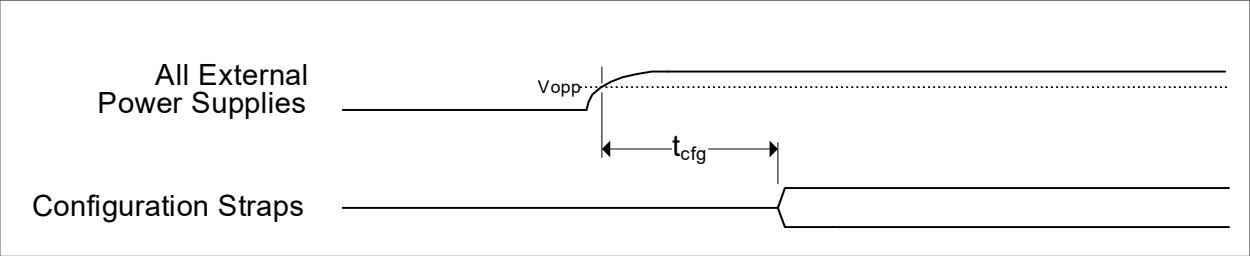
FIGURE 18-5: POWER-ON CONFIGURATION STRAP LATCHING TIMING
