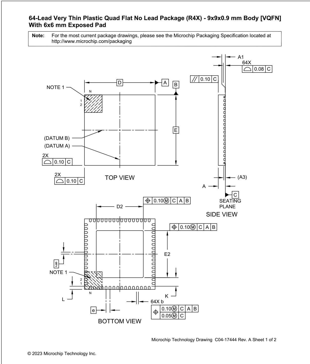
FIGURE 19-1: 64-QFN PACKAGE DRAWING
