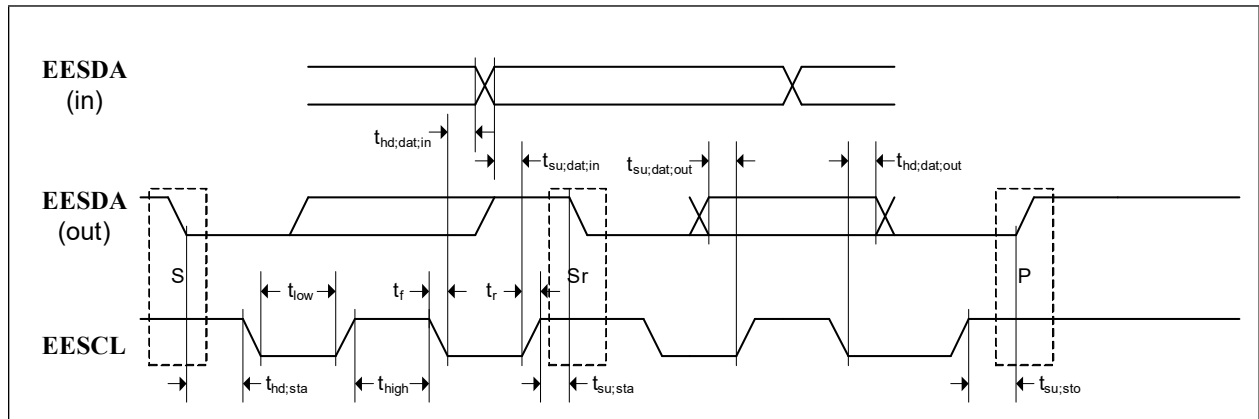
FIGURE 13-1: I 2 C CONTROLLER TIMING DIAGRAM
