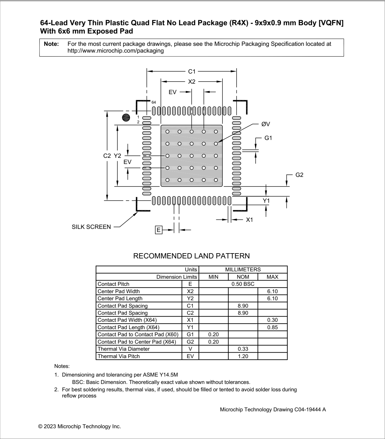
FIGURE 19-3: 64-QFN PACKAGE LAND PATTERN
