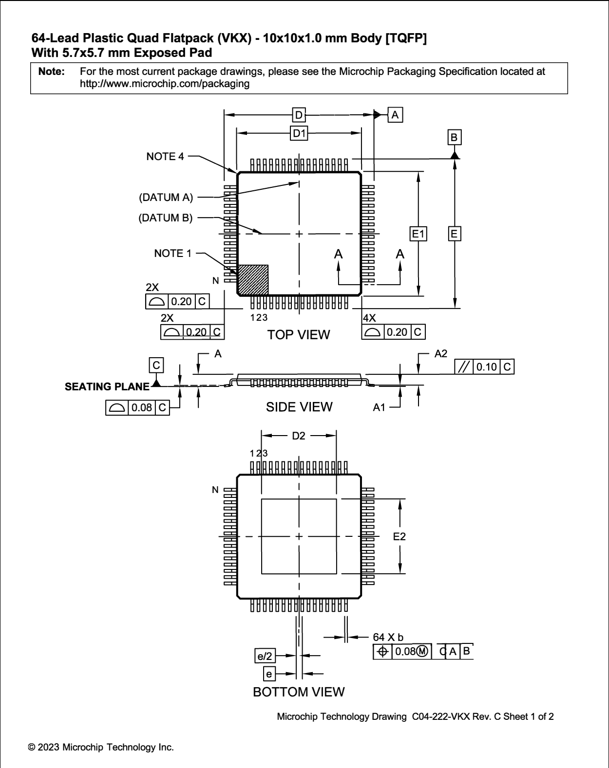
FIGURE 20-4: 64-TQFP-EP DRAWING
