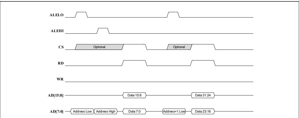
FIGURE 9-4: MULTIPLEXED ADDRESSING WITH DUAL PHASE LATCHING - 16-BIT READ WITHOUT ALEHI
