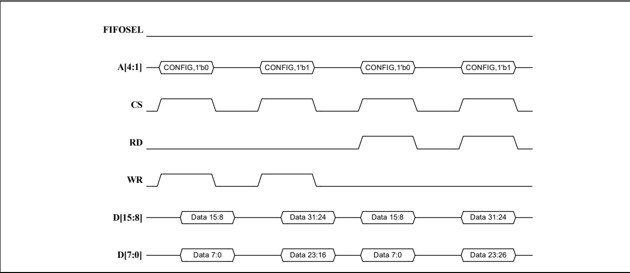
FIGURE 9-25: INDEXED ADDRESSING CONFIGURATION REGISTER ACCESS - 16-BIT WRITE/ READ
