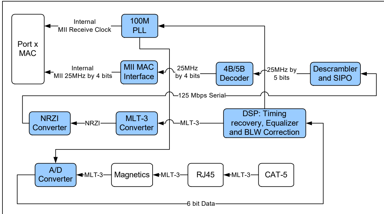
FIGURE 12-3: 100BASE-TX RECEIVE DATA PATH
