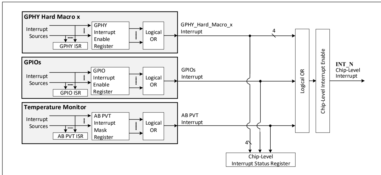
FIGURE 5-8: INTERRUPT STRUCTURE
