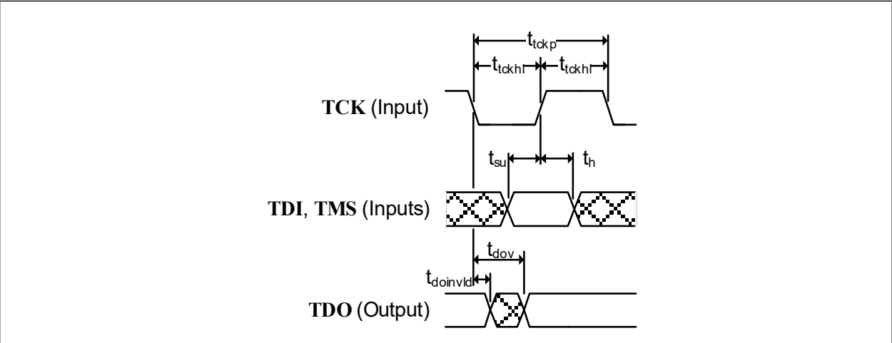
FIGURE 6-6: JTAG TIMING
