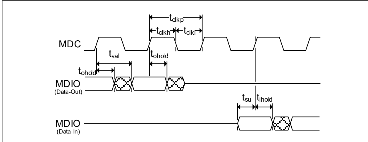
FIGURE 6-5: MDC/MDIO TIMING
