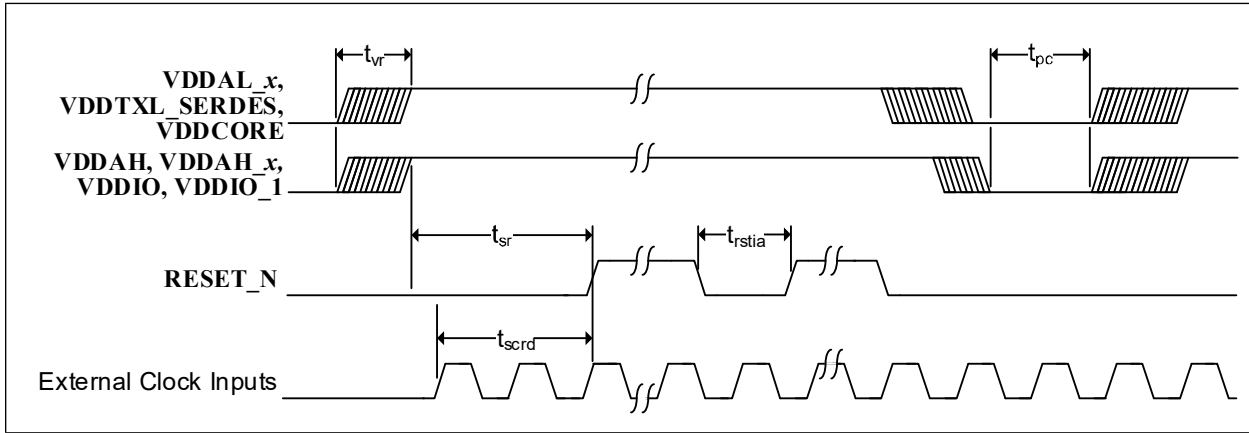
FIGURE 6-2: POWER SEQUENCE TIMING INTERNAL REGULATORS
