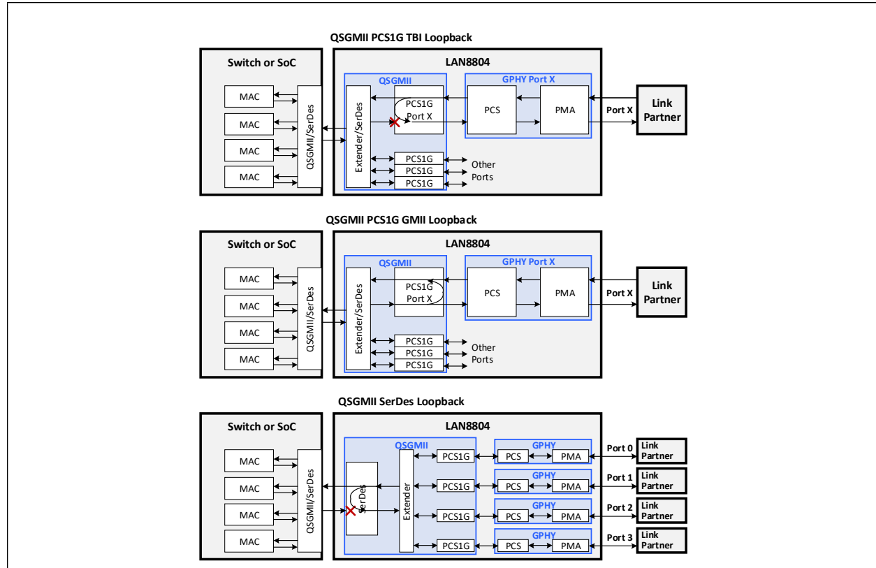
FIGURE 5-6: QSGMII LOOPBACK
