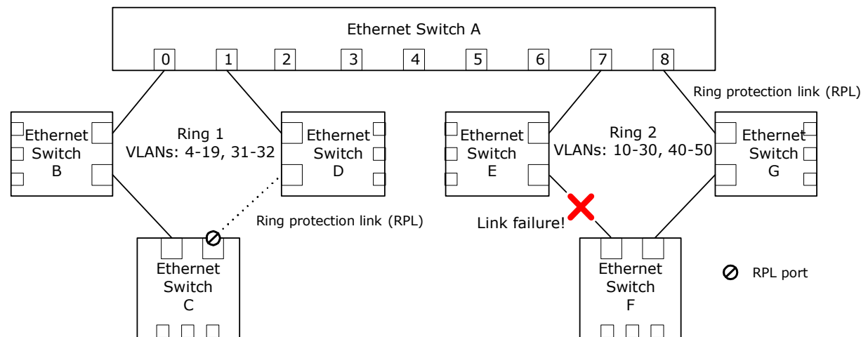
FIGURE 2-118: ETHERNET RING WITH FAILURE
