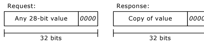
FIGURE 2-111: IDLE COMMAND
