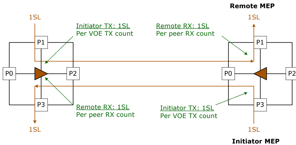
FIGURE 2-57: DUAL-ENDED SYNLM
