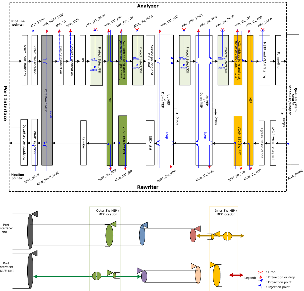
FIGURE 2-11: PROCESSING FLOW
