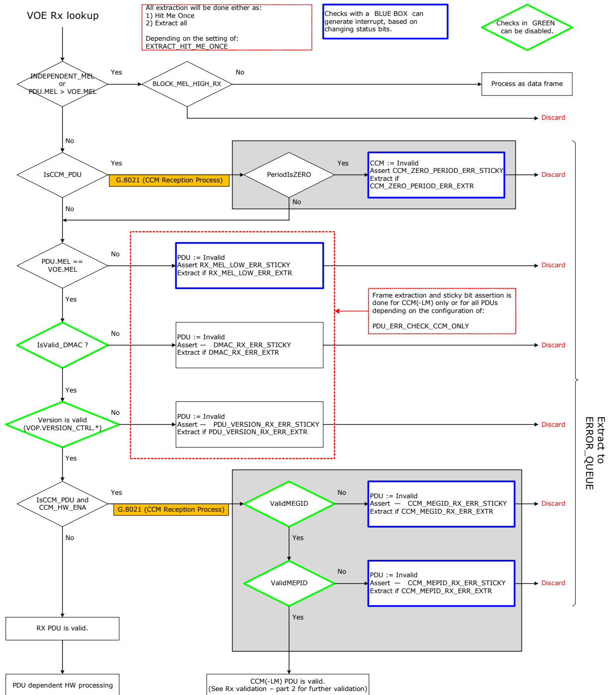
FIGURE 2-54: RX VALIDATION, PART 1
