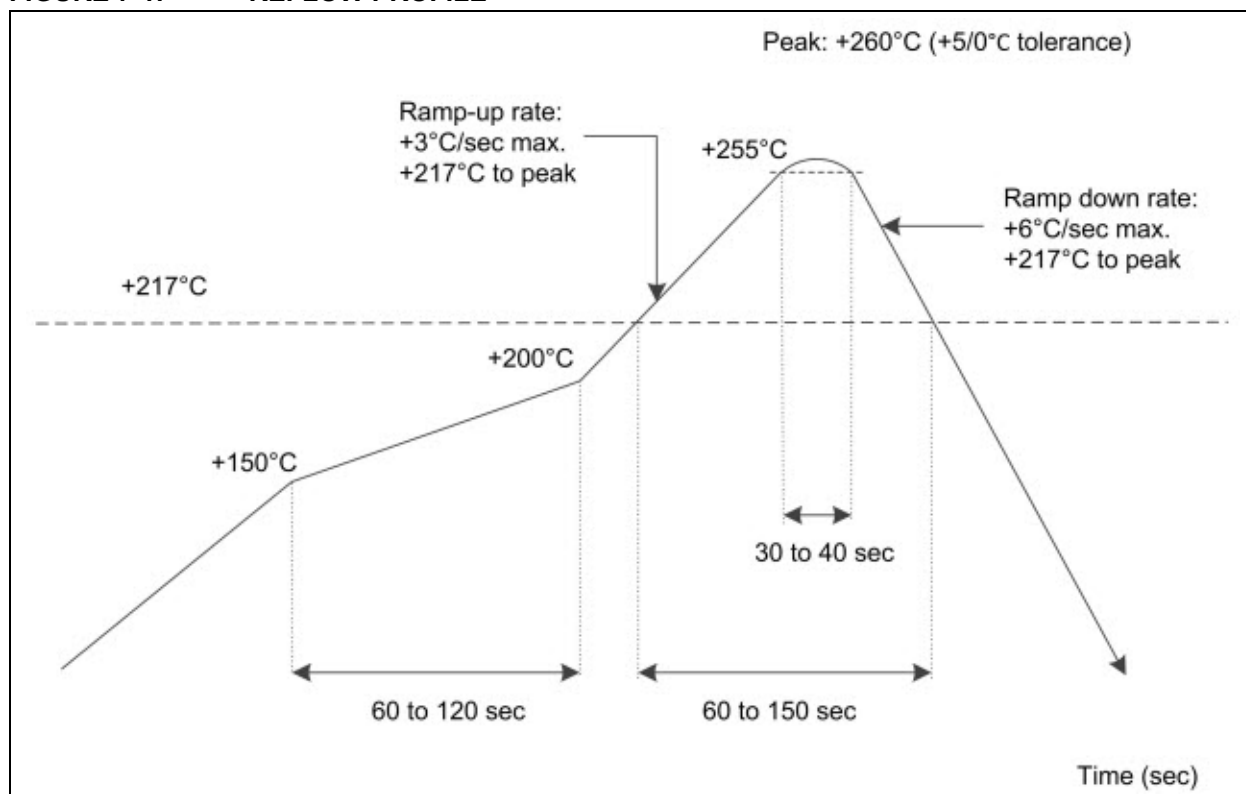
FIGURE 7-1: REFLOW PROFILE
