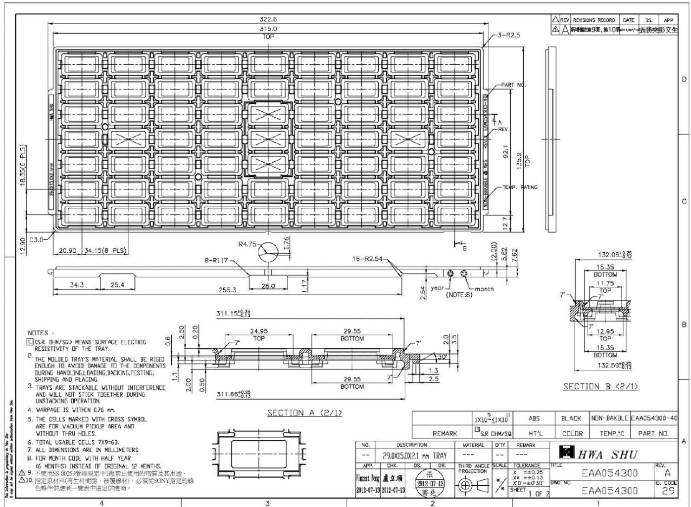
Figure 7-2. Packaging Information
