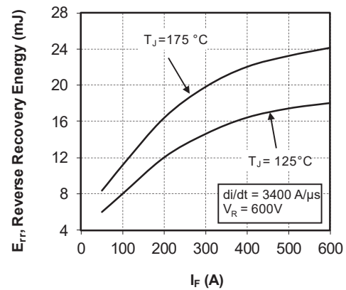
Figure 3-3. Energy Losses vs. Forward Current
