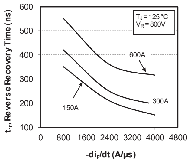
Figure 3-3. t_{rr} vs. Current Rate of Charge
