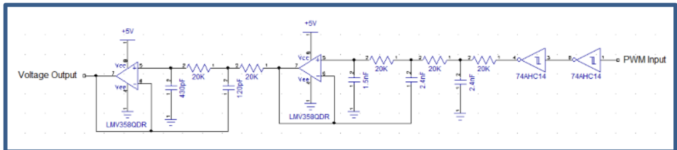
Figure 12 Example of a 2kHz Low Pass Filter
