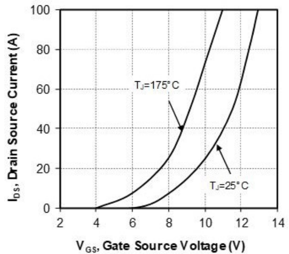
Figure 1-5. Transfer Characteristics
