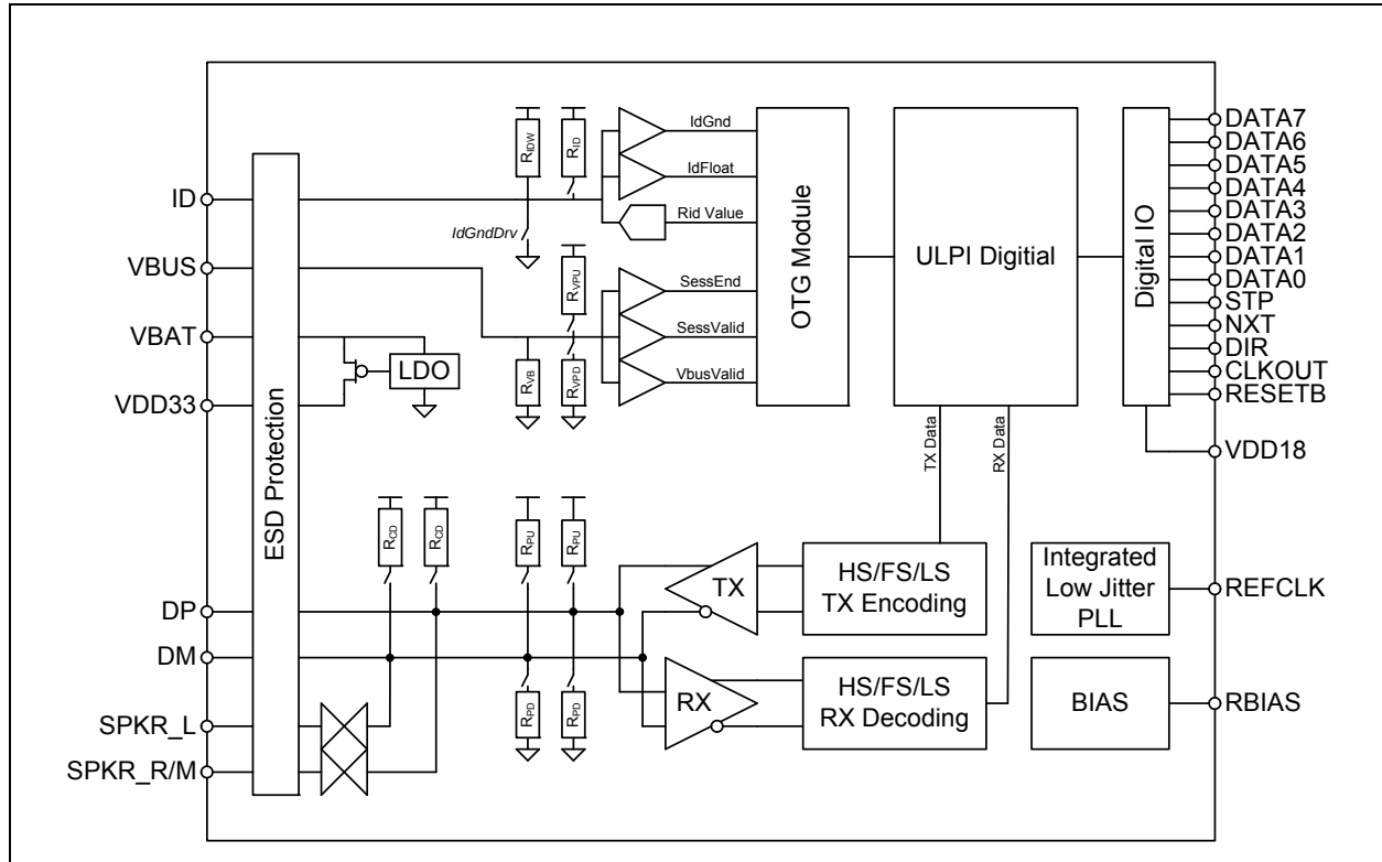
FIGURE 5-1: USB3316 SYSTEM DIAGRAM
