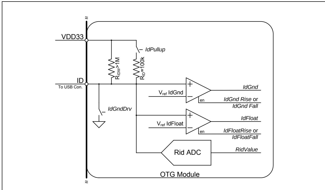
FIGURE 5-8: USB3316 ID RESISTOR DETECTION CIRCUITRY
