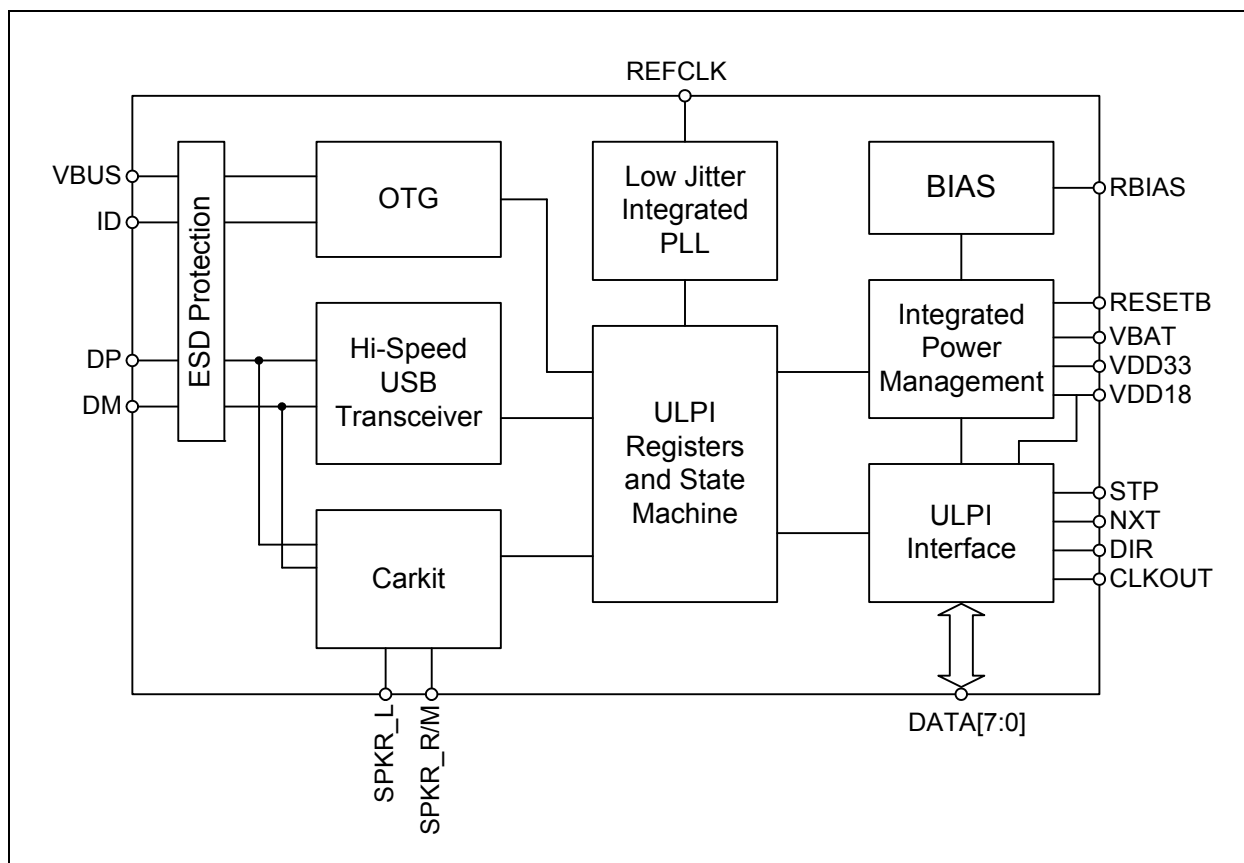
FIGURE 1-1: USB3316 BLOCK DIAGRAM
