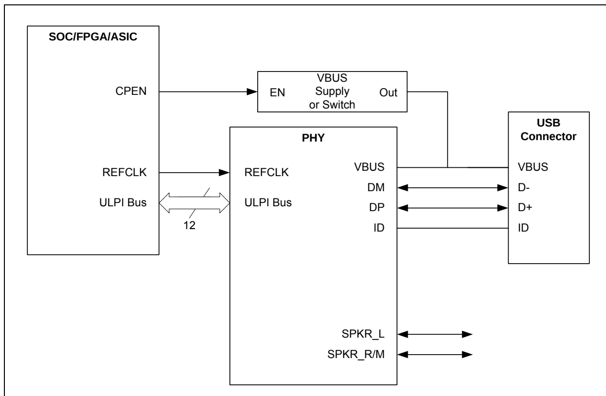
FIGURE 5-10: OTG LINK CONTROLLER DRIVES EXTERNAL VBUS SUPPLY OR SWITCH
