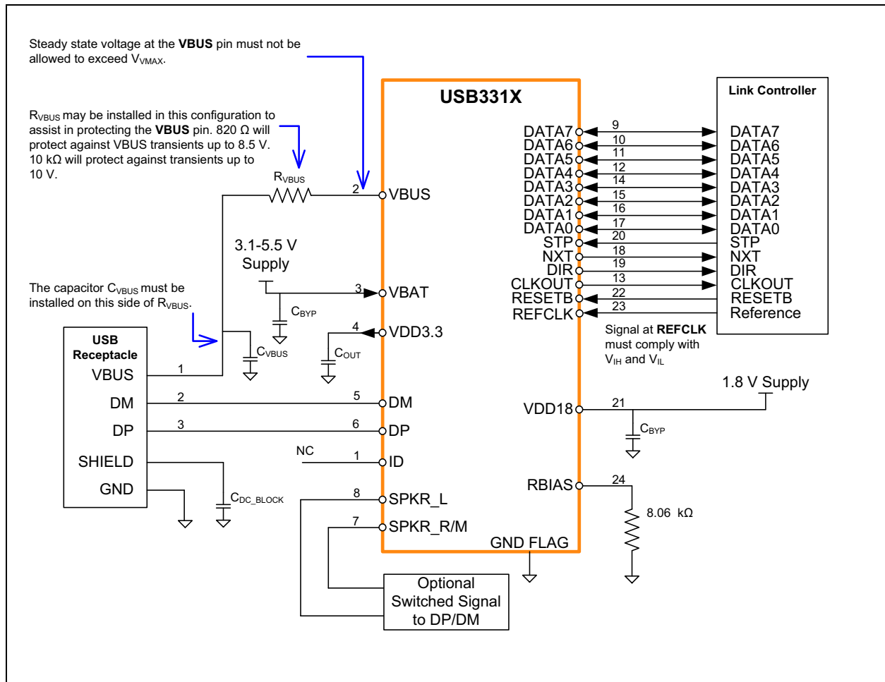
FIGURE 8-1: USB3316 QFN APPLICATION DIAGRAM (DEVICE)
