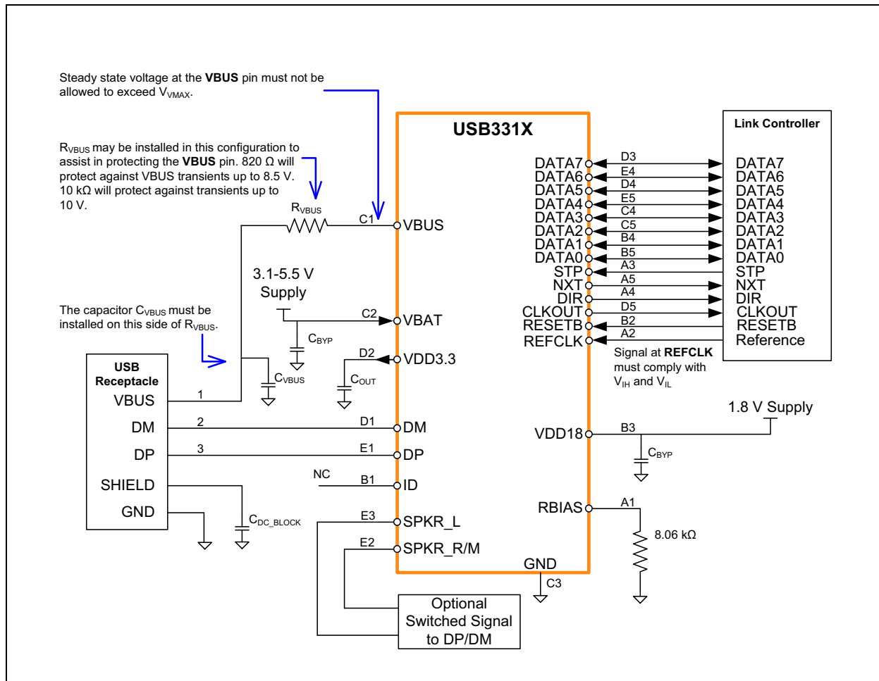
FIGURE 8-2: USB3316 BGA APPLICATION DIAGRAM (DEVICE)
