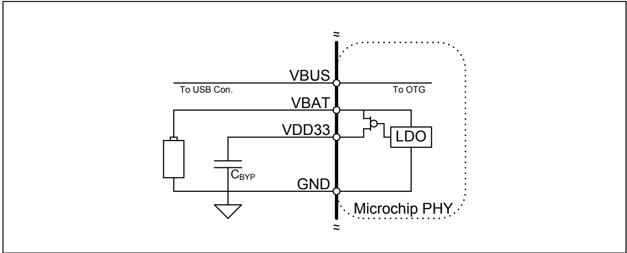
FIGURE 5-4: POWERING THE USB3316 FROM A BATTERY
