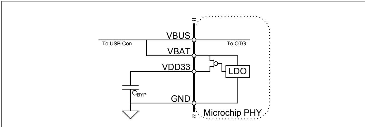
FIGURE 5-6: POWERING THE USB3316 FROM THE USB CABLE VBUS
