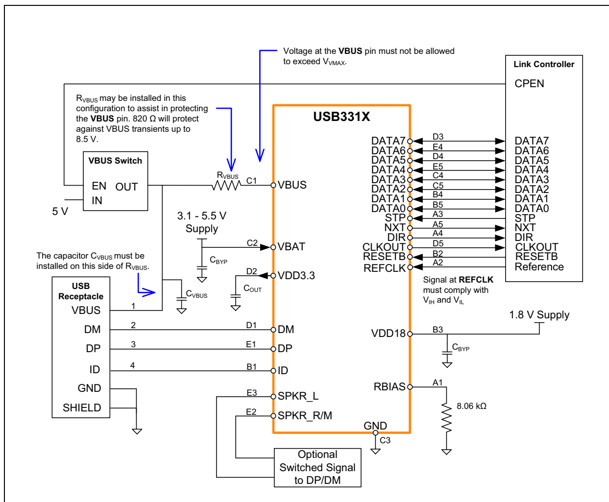
FIGURE 8-4: USB3316 BGA APPLICATION DIAGRAM (HOST OR OTG)
