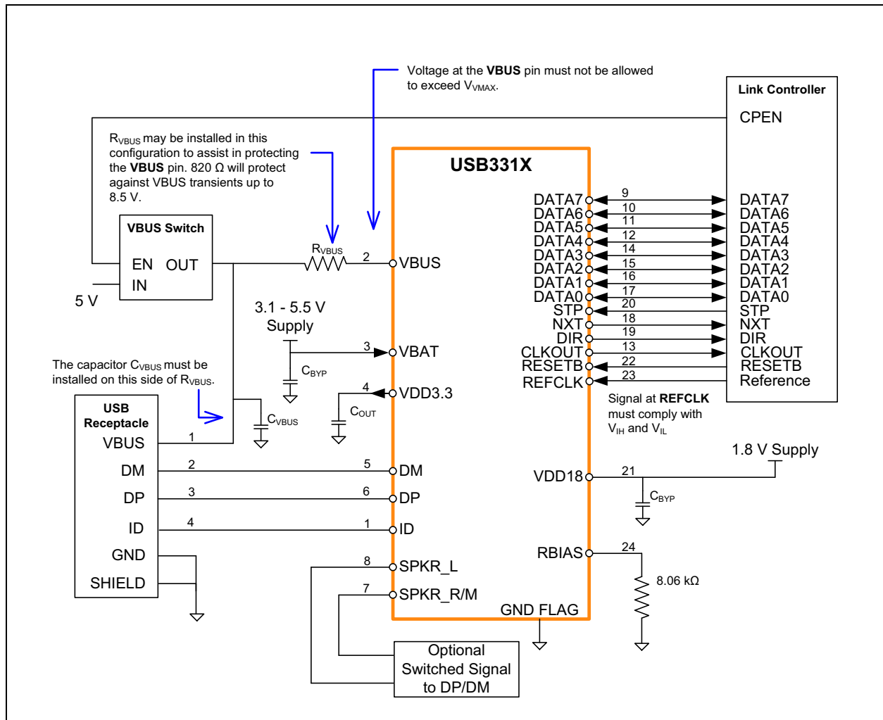
FIGURE 8-3: USB3316 QFN APPLICATION DIAGRAM (HOST OR OTG)
