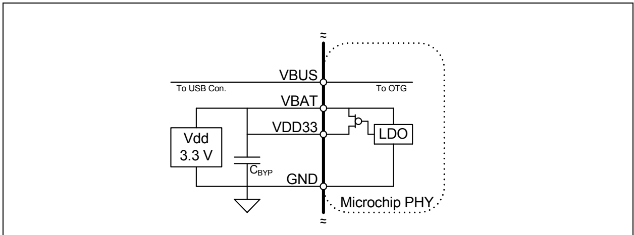
FIGURE 5-5: POWERING THE USB3316 FROM A 3.3 V SUPPLY
