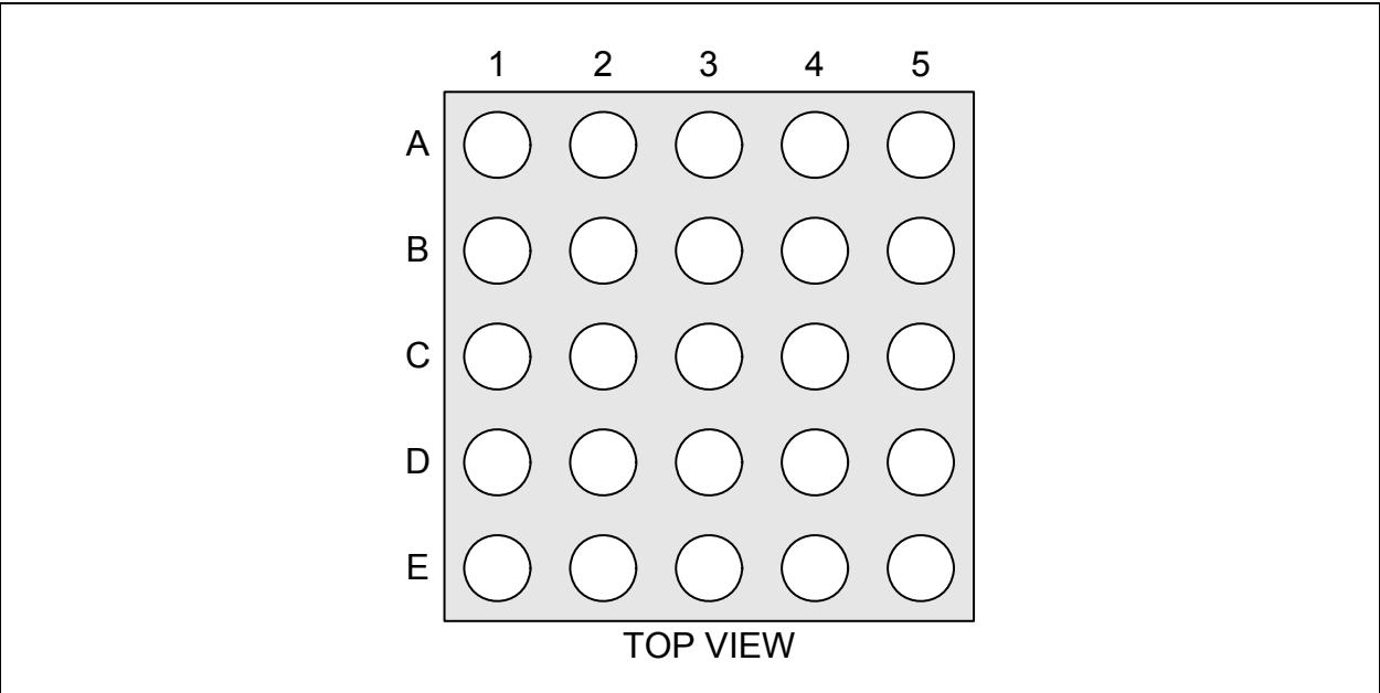
FIGURE 2-2: USB3316 VFBGA PINOUT - TOP VIEW
