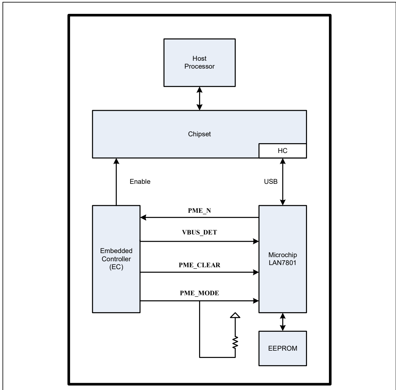
FIGURE 13-1: TYPICAL APPLICATION
