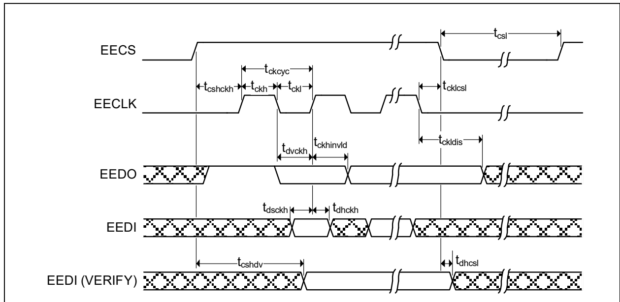
FIGURE 15-9: EEPROM TIMING
