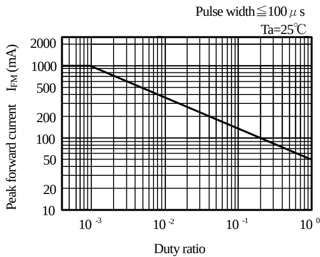
(Fig. 5) Peak forward current vs. Duty ratio
