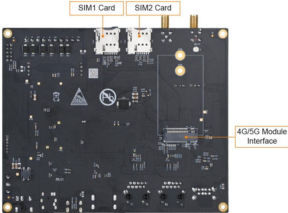
MYD-LMX9X Development Board (Bottom view)
